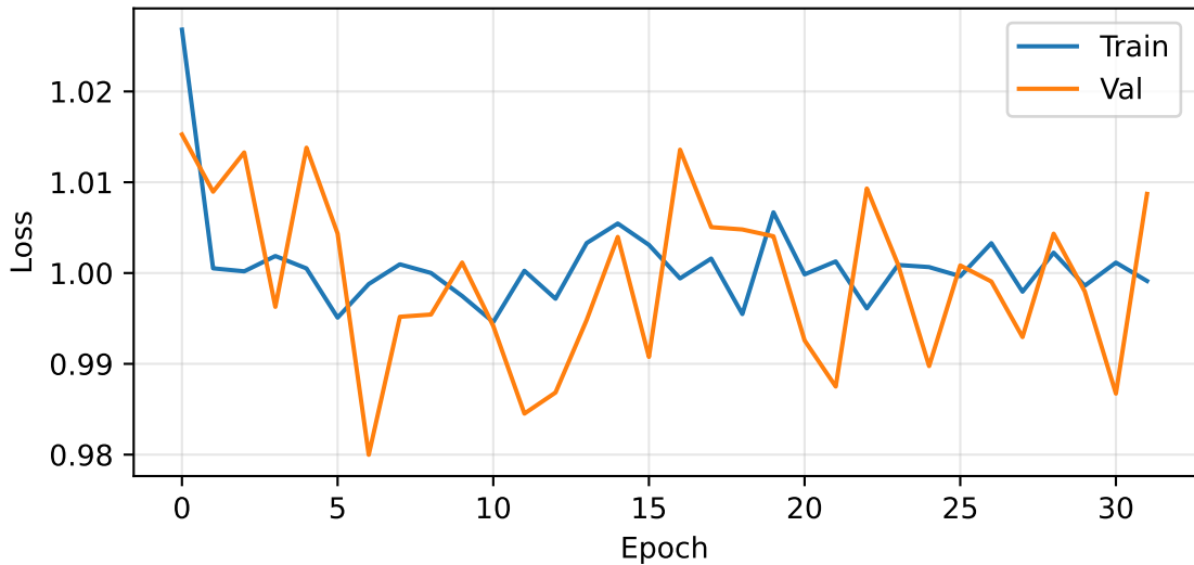
Losses: ddpm_evaluation_20250813_114721
